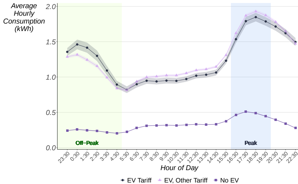
Figure 3: Pre-Trial (January 2024) Hourly Consumption
