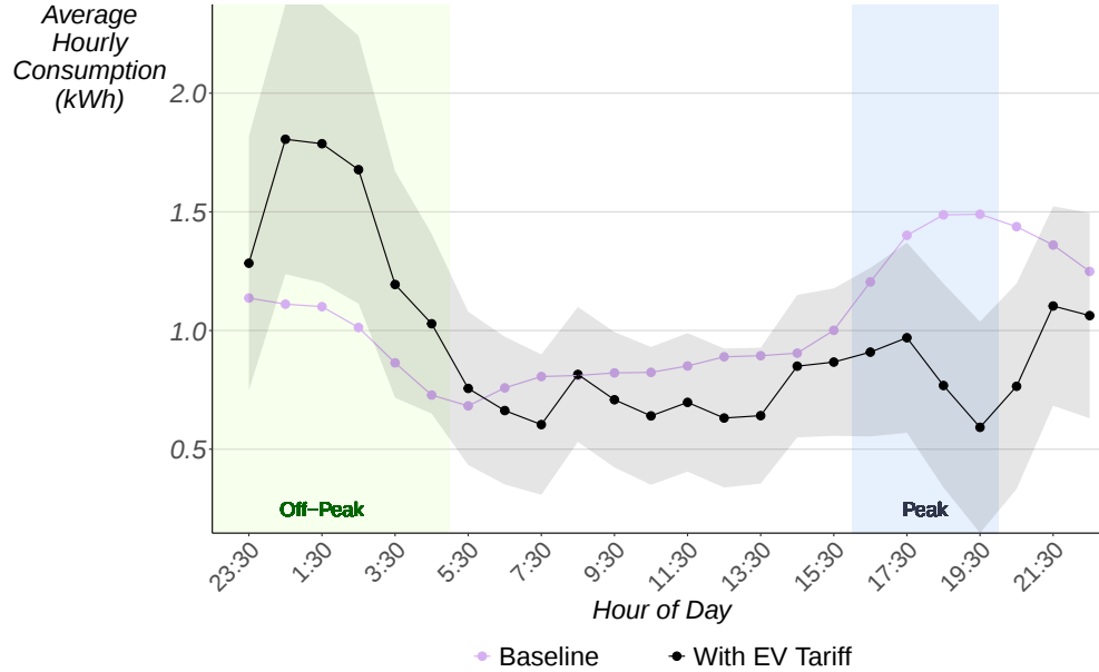
Figure 7: Electricity Consumption With and Without EV Tariff Adoption
