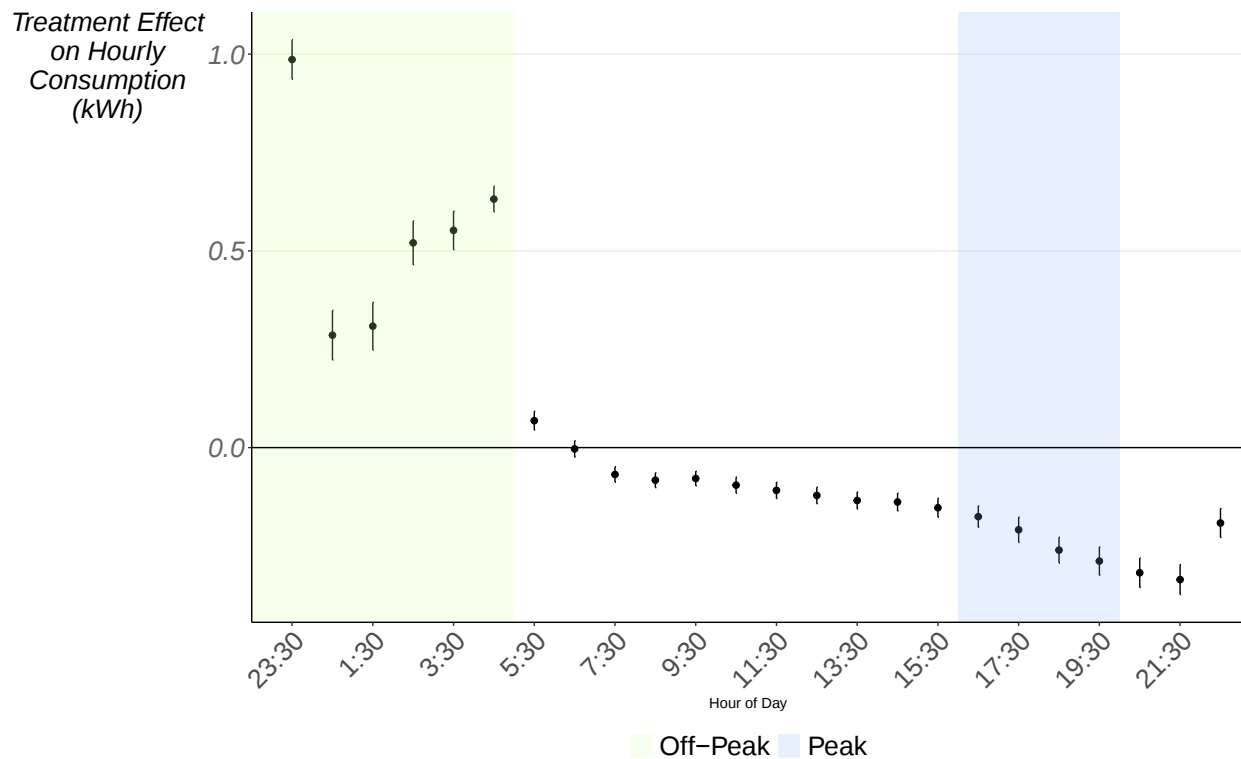
Figure A13: Difference-in-Differences Estimate of IO Go, by Hour-of-day
