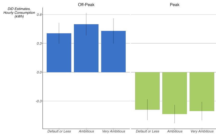
Figure A19: Estimated Impact of IO GO, by User Preferences
