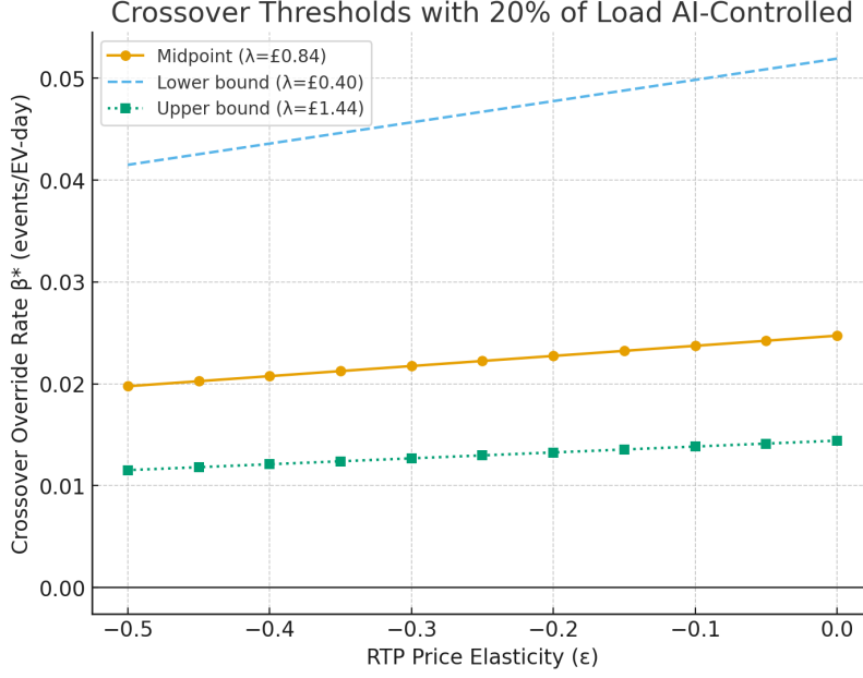
Figure 25: Crossover override thresholds
