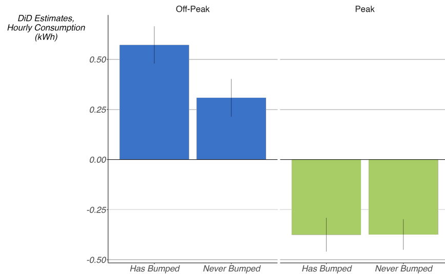
Figure A18: Estimated Impact of IO GO, by “Bump” (Override) Behavior
