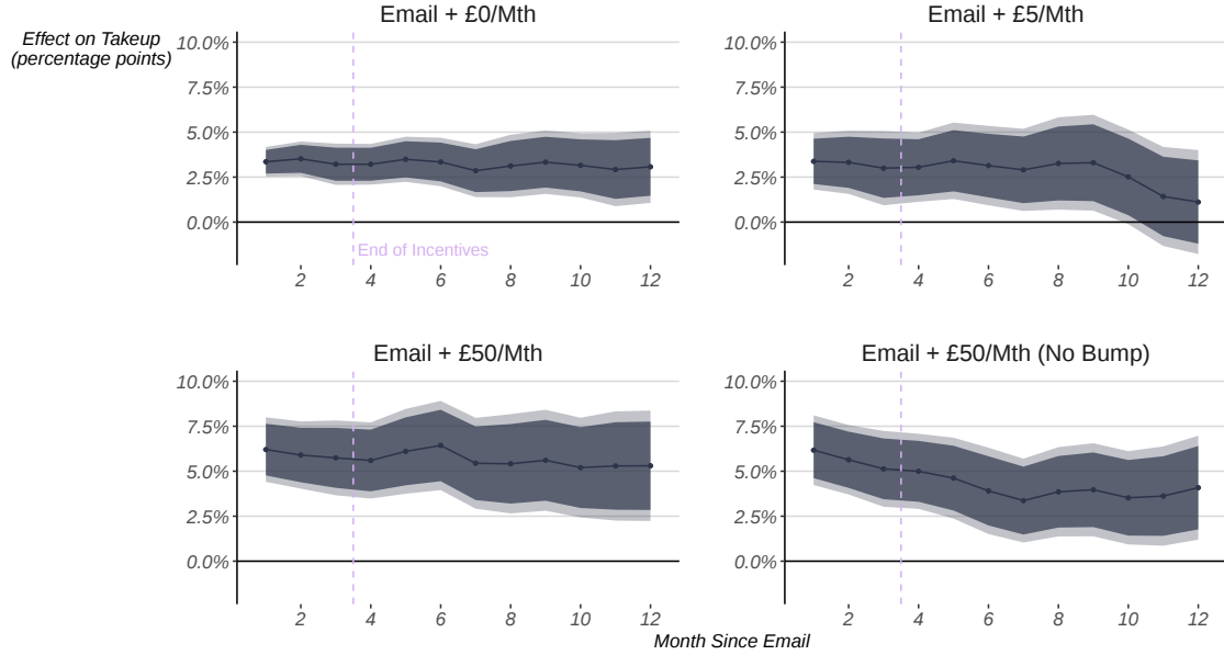
Figure 4: Impact of Encouragements on Take-up of Managed Charging Tariff (IO Go)
